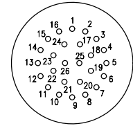
CONTACT CONFIGURATION (BCR FACE VIEW)
