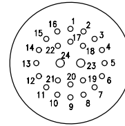
CONTACT CONFIGURATION (BCR FACE VIEW)
